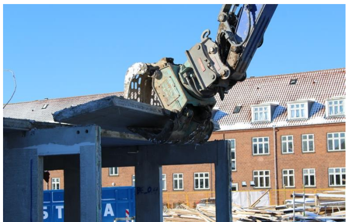
Figure 8 Dismantling of concrete element for re-use (Source: Danish Technological Institute)
